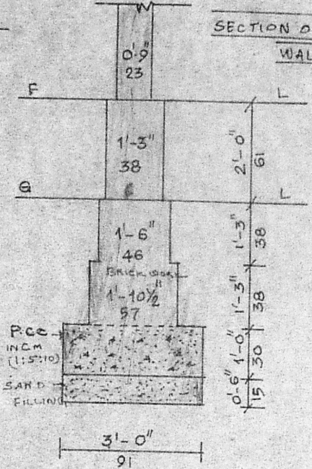
FOUNDATION DETAIL [SCALE 1" = 2'-0"]
