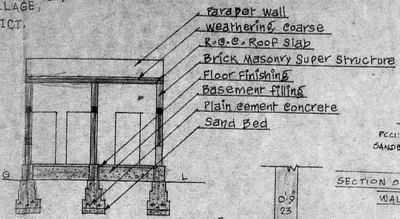
SECTION AT-XX
