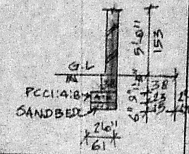
SECTION OF COMPOUND WALL
